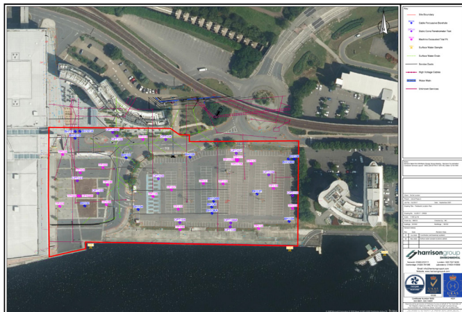
Site plan showing intrusive investigation positions
